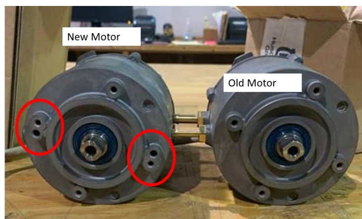
Figure 1: New Motor with steering pins.
