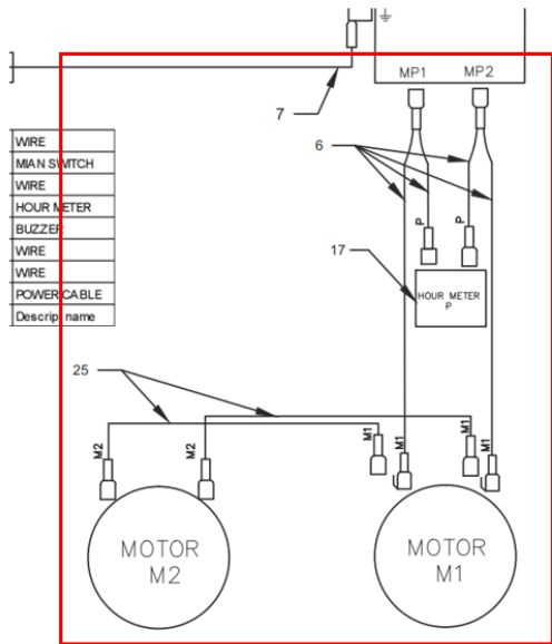
Old motor cables schematic.
