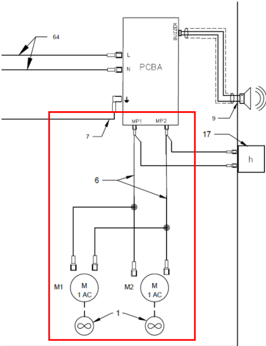
New motor cable schematic.
