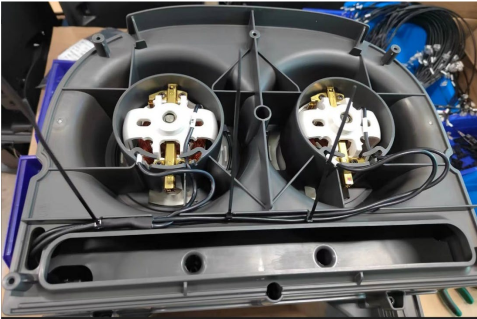
Motor cables are routed as picture. Make sure the splice fits inside the groove.
