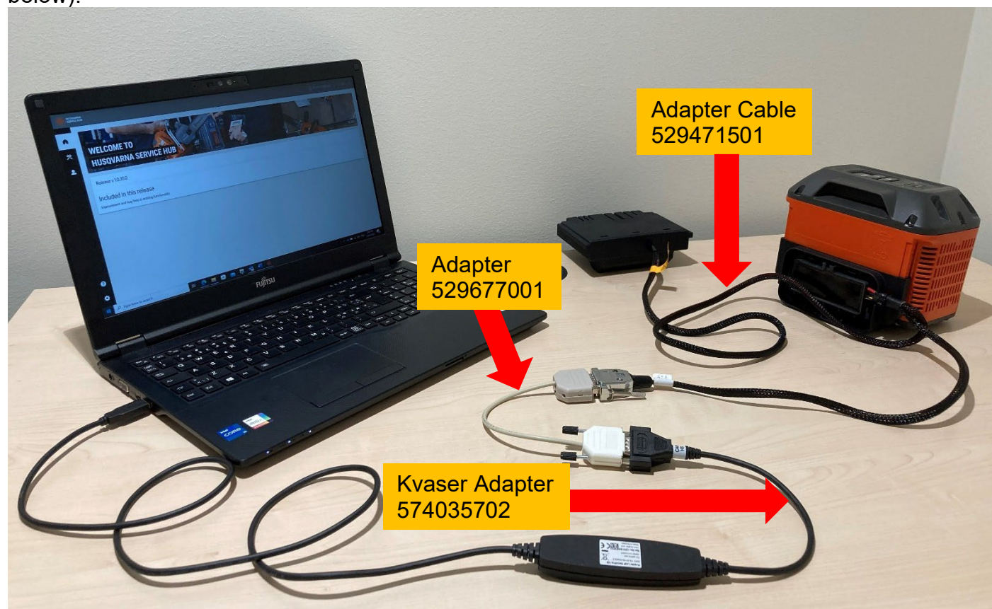
Figure 2: Connecting Pace battery to Husqvarna Service Hub without Interface Box
