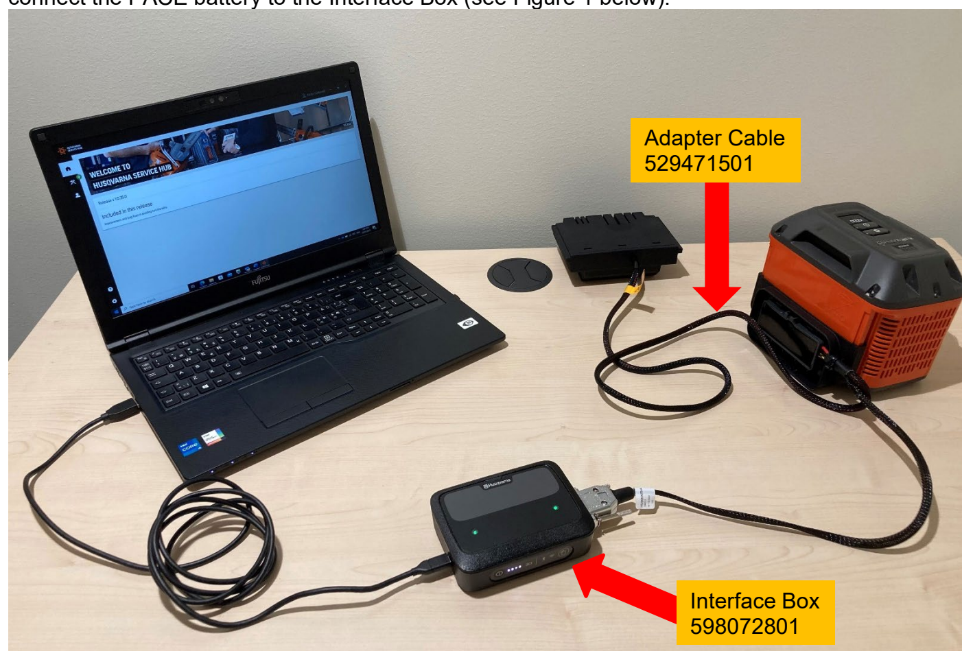
Figure 1: Connecting Pace battery to Husqvarna Service Hub using Interface Box
