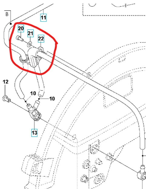
Figure 2: WATER HOSE HOLDER introduced on 14".
