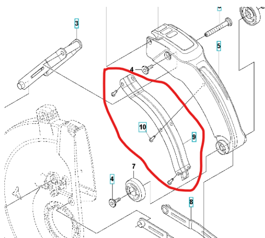
Figure 1: Wear Plate introduced on 14".
