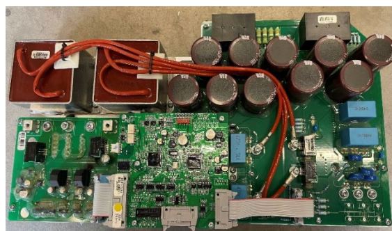
Figure 1: Inverter board.
