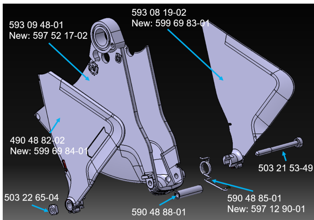
Figure 2: Old Movable blade guard.
