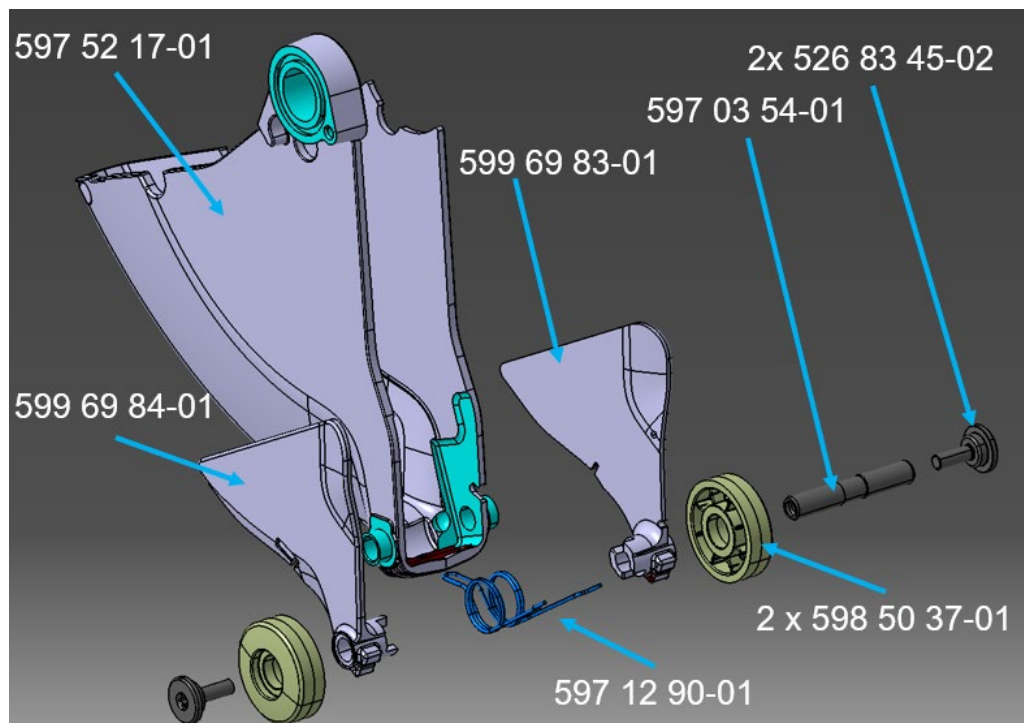
Figure 1: New Movable Blade Guard.
