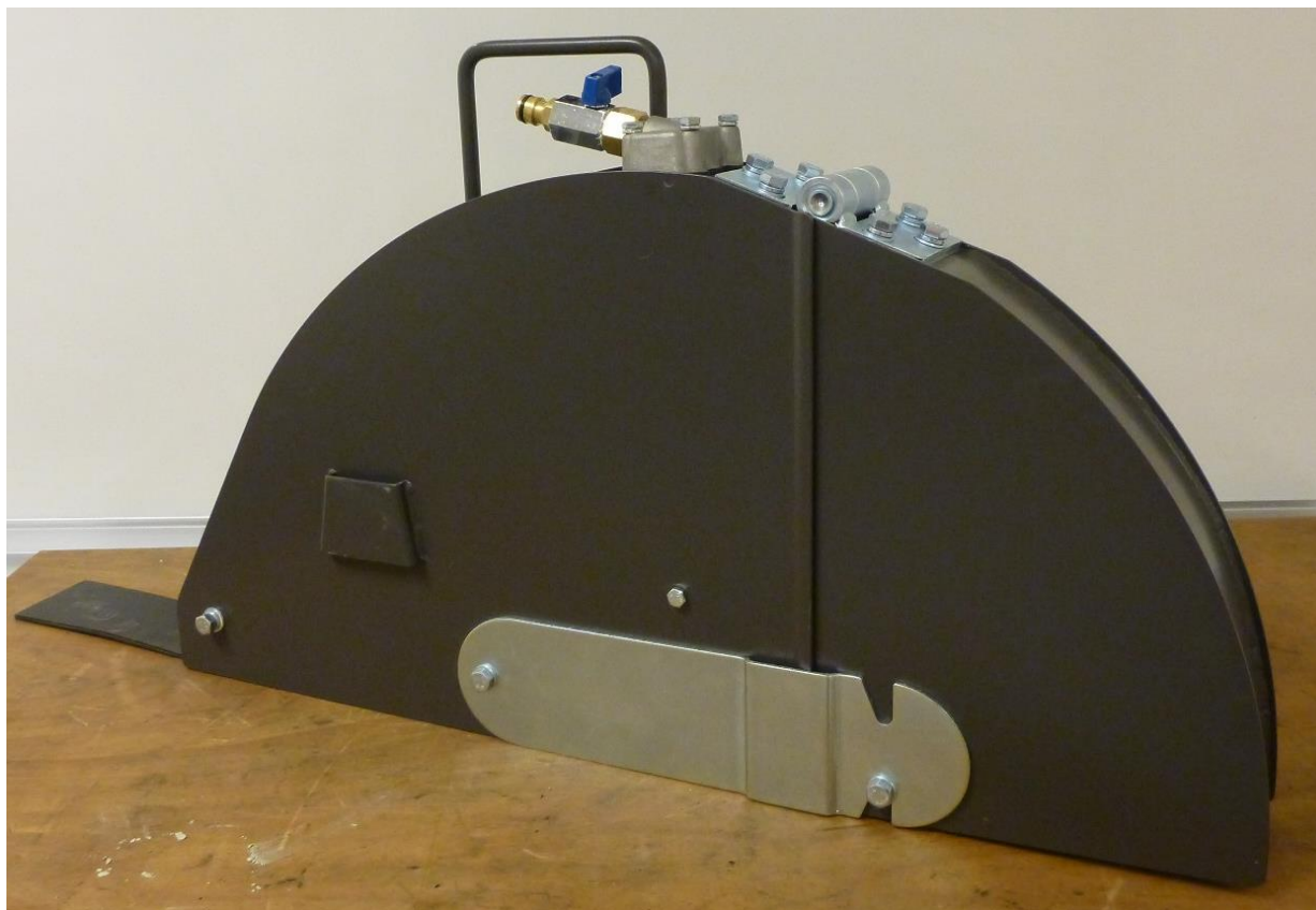
Figure 3: New blade guard design. 20" / 500 mm (501 12 59-01).
