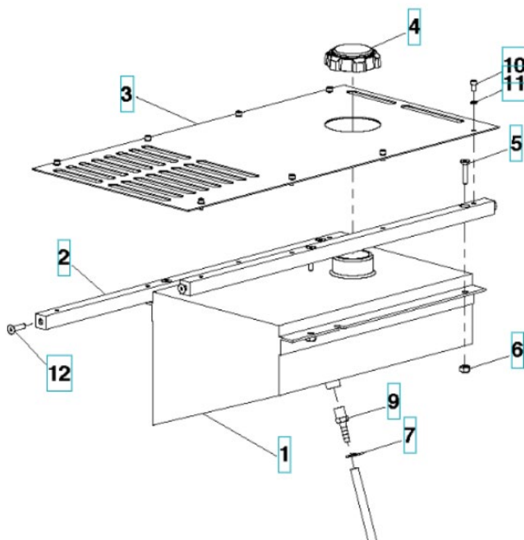
Figure 1: Updated fuel tank and cover.
