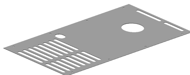
Figure 3: Updated Cover Soff-Cut 4200 – 577608502
